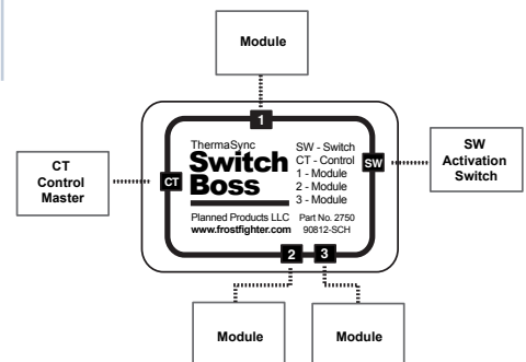
Switch Boss with Master CT and Modules
