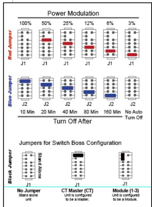
Jumper guide for ThermaSync Controls showing the jumpers for each function. Not all controls have color coded jumpers.
